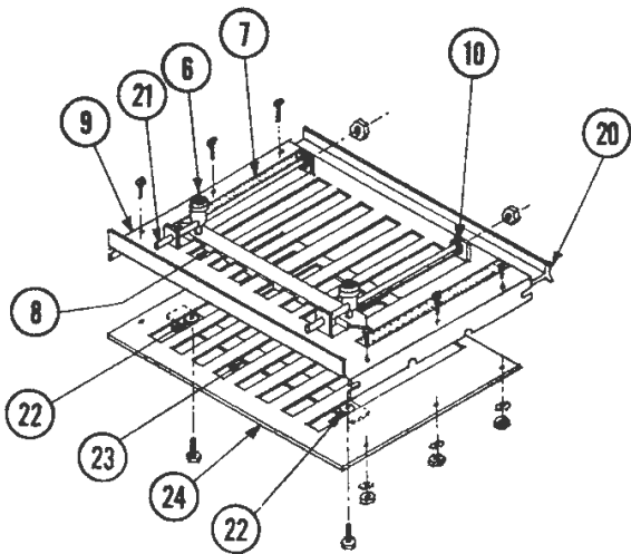
Assembly 251X, Upper and Lower Fold Tables Complete - WRA095101
