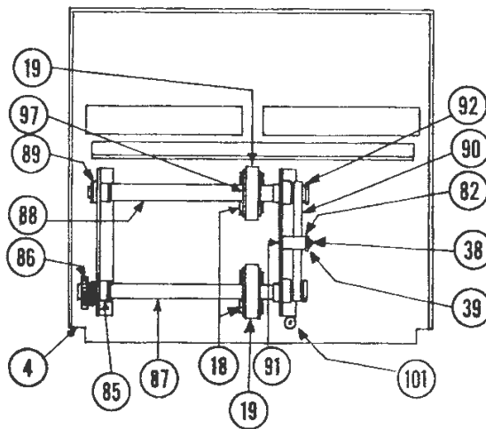
Feed Table 354X Parts Detail
